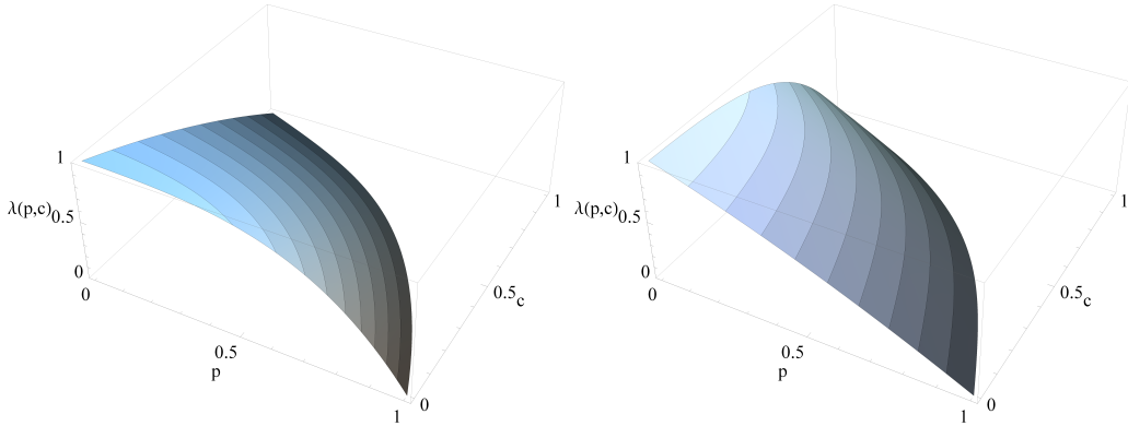
Figure 1: Graphs of \lambda_1 (on the left) and \lambda_2 (on the right).
